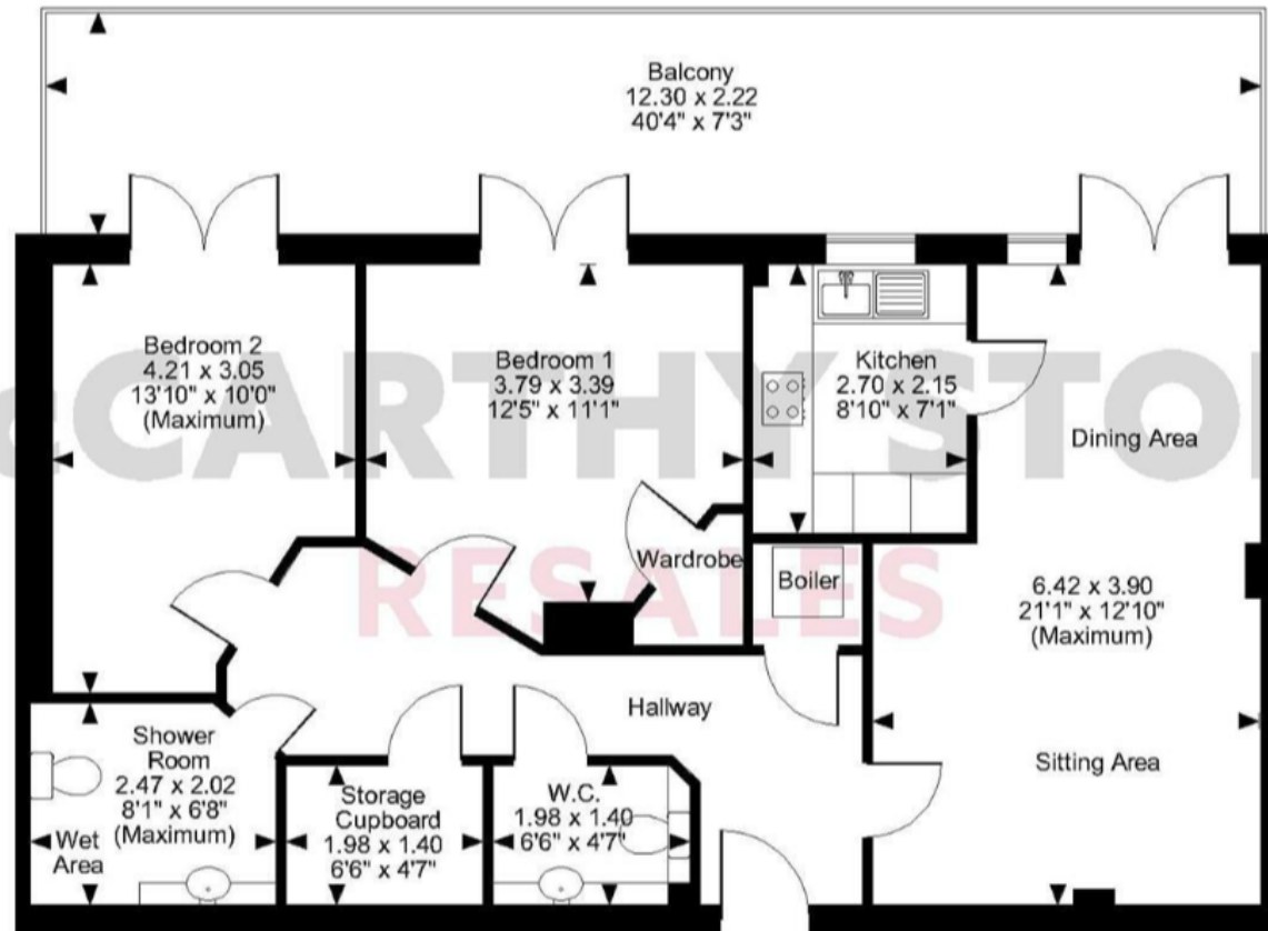
Third Floor
