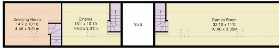
First Floor
