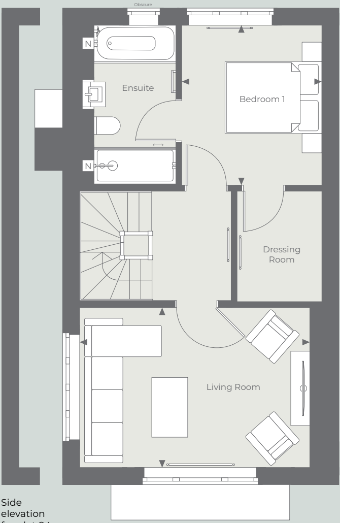
First Floor
