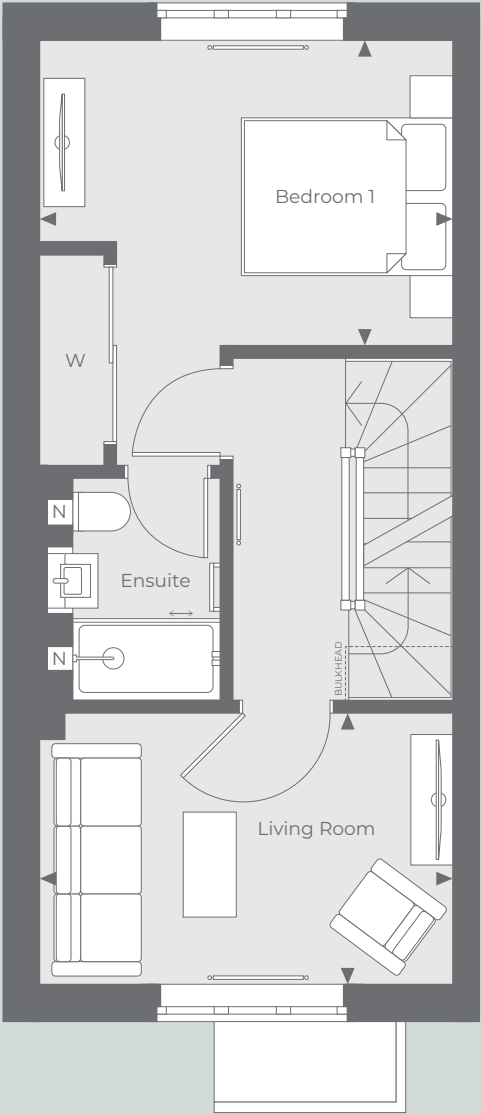
First Floor
