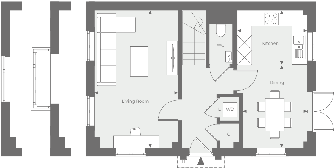
Ground Floor
