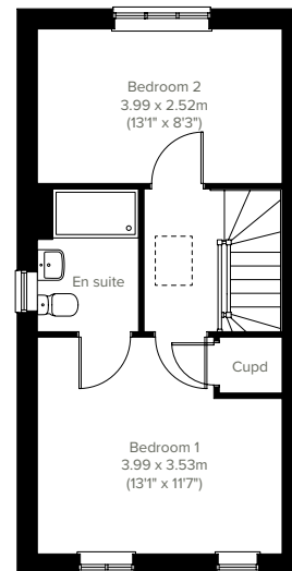
2ND FLOOR
