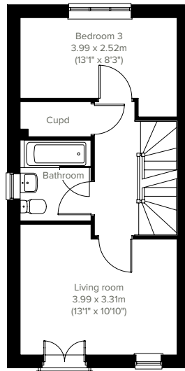
1ST FLOOR
