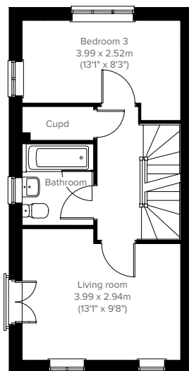
1ST FLOOR
