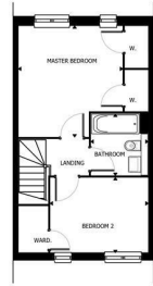
First Floor Plan Layout Scale 1:100
