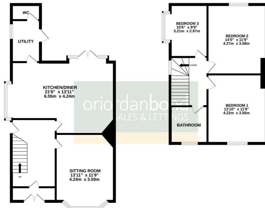
GROUND FLOOR 664 sq.ft. (61.6 sq.m.) approx.
