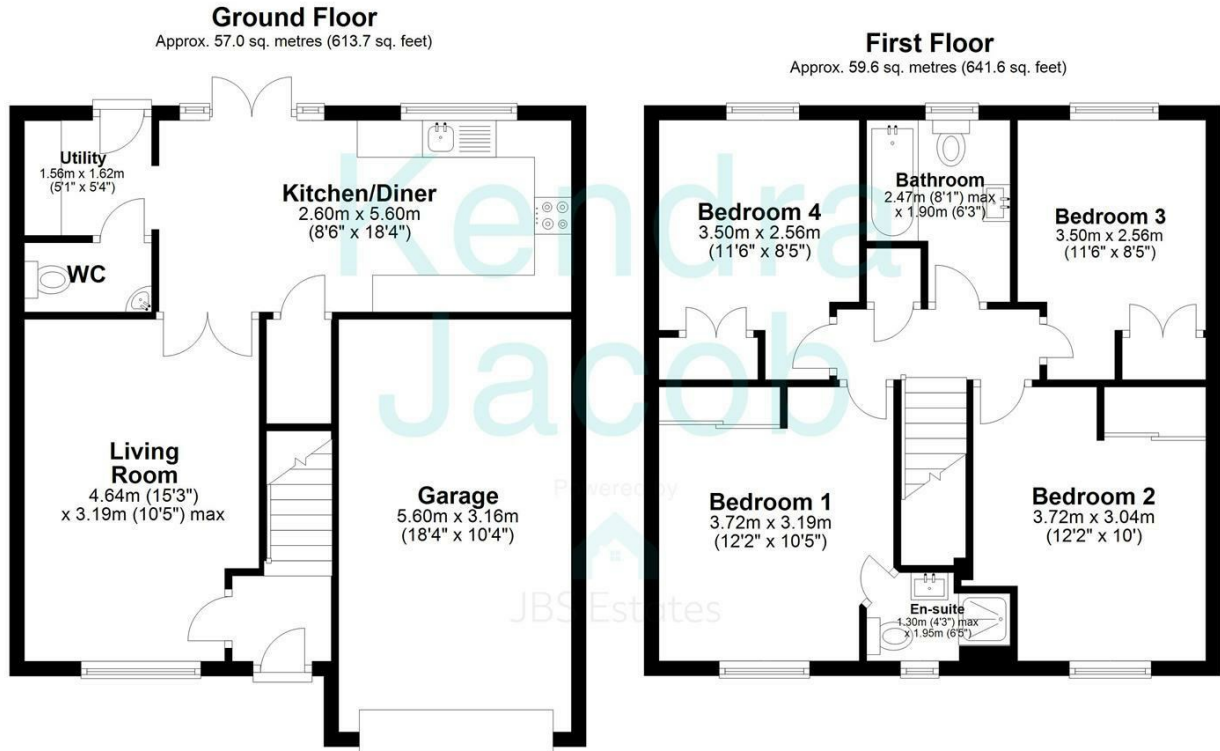
Total area: approx. 116.6 sq. metres (1255.3 sq. feet) Illustration for identification purposes only, measurements are approximate, not to scale. Plan produced using PlanUp.
