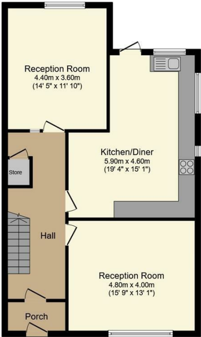
Ground Floor Floor area 74.1 sq.m. (798 sq.ft.)
