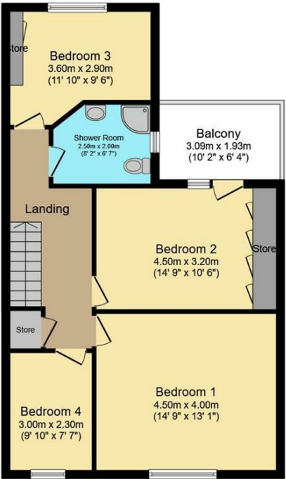
First Floor Floor area 65.2 sq.m. (701 sq.ft.)
