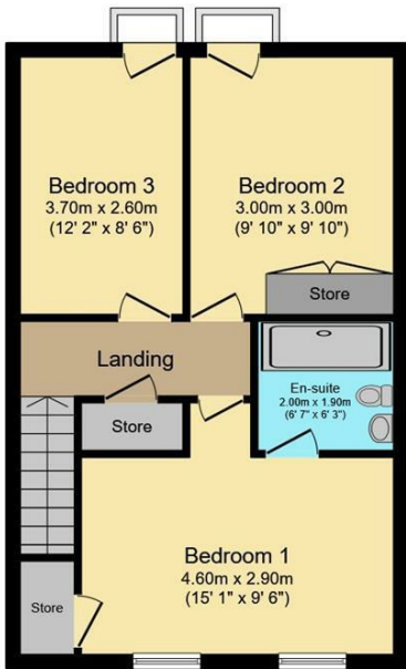
Second Floor Floor area 48.3 sq.m. (520 sq.ft.)
