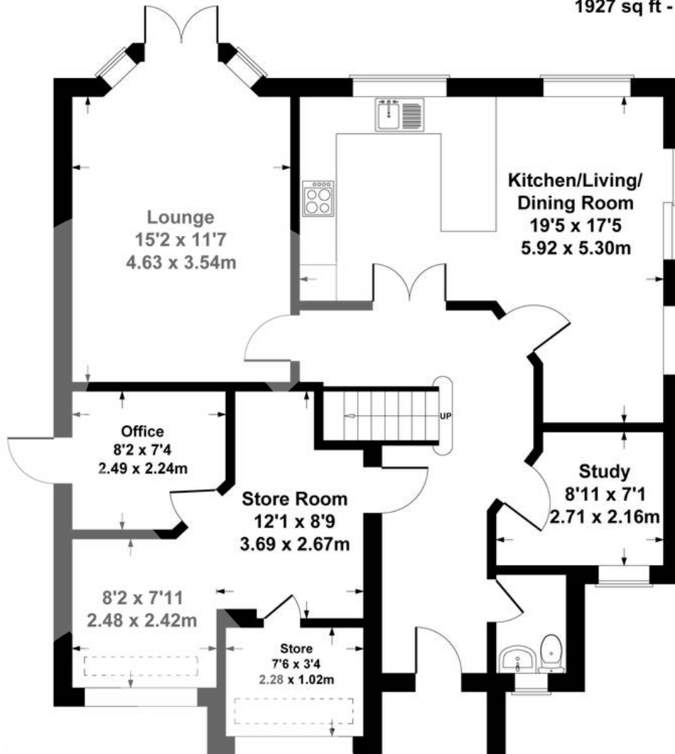
GROUND FLOOR
