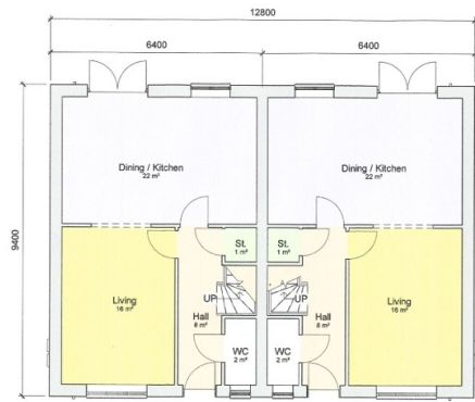
1 00 Ground Floor NTS
