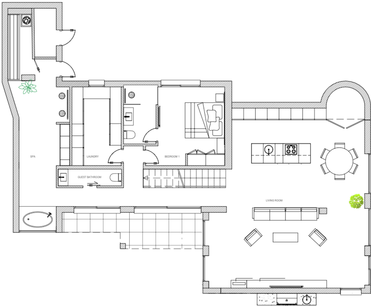
GROUND FLOOR
