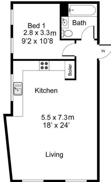
FIRST FLOOR FLAT
