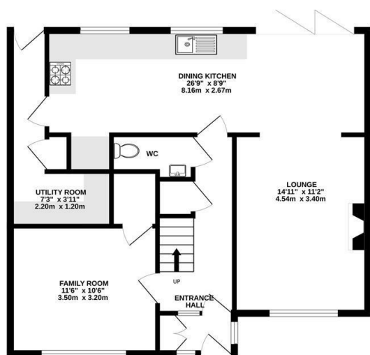
GROUND FLOOR 763 sq.ft. (70.9 sq.m.) approx.
