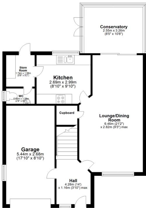
Ground Floor Approx. 65.7 sq. metres (707.7 sq. feet)
