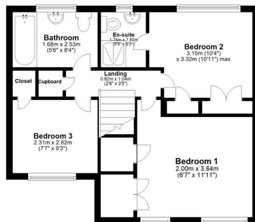
First Floor Approx. 45.0 sq. metres (484.2 sq. feet)
