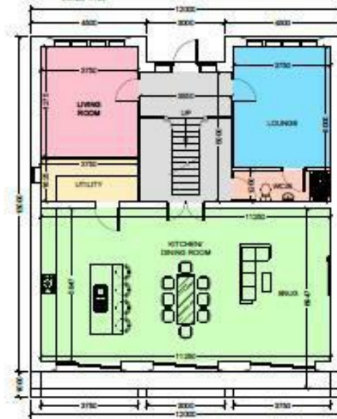
PLOT 1 GROUND FLOOR PLAN
