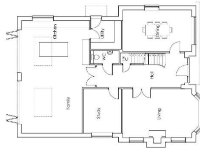
Ground Floor Plan 1:100
