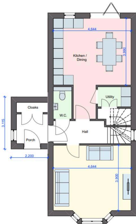
PROPOSED GROUND FLOOR LAYOUT
