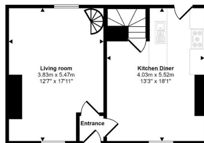
Ground Floor Approx 44 sq m / 476 sq ft
