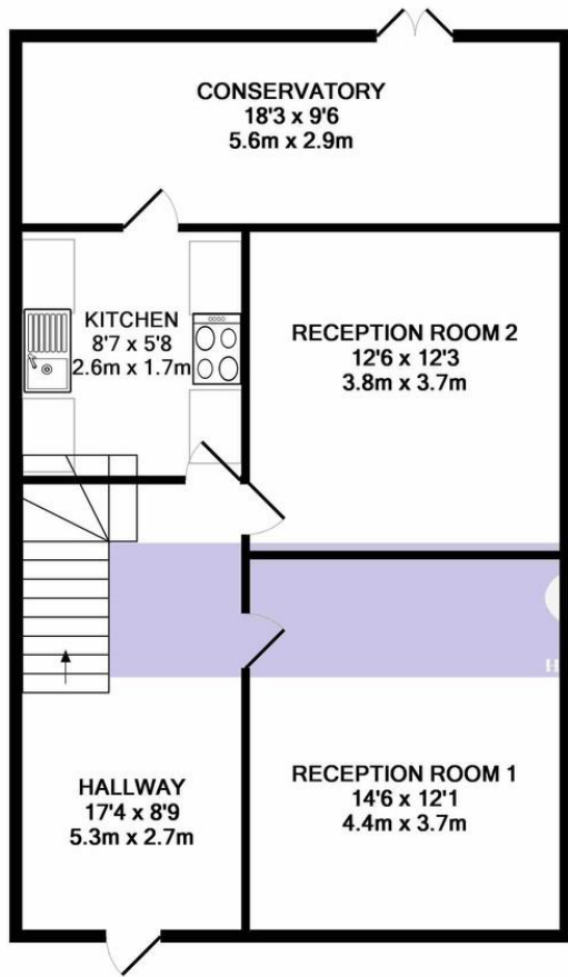
GROUND FLOOR APPROX. FLOOR AREA 714 SQ.FT. (66.4 SQ.M.)
