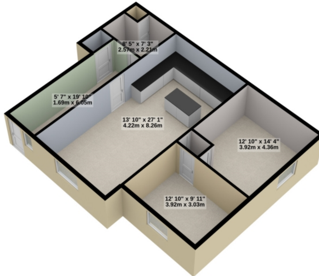
GROUND FLOOR 870 sq.ft. (80.8 sq.m.) approx.
