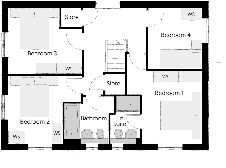
First Floor
