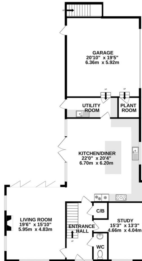
GROUND FLOOR 1593 sq.ft. (148.0 sq.m.) approx.
