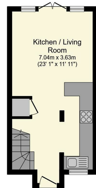
Ground Floor Floor area 26.2 m 2 (282 sq.ft.)
