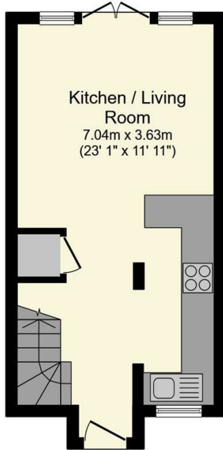
Ground Floor Floor area 26.2 m 2 (282 sq.ft.)
