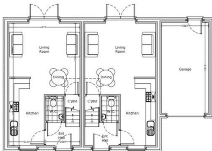
Proposed Ground Floor Plans Gross Floor Area = 63m 2 or 678ft 2 (Exc. Garage) Garage Gross Floor Area = 15.5m 2 or 166ft 2
