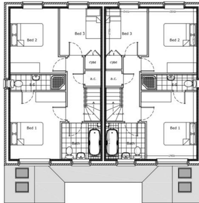
Proposed First Floor Plans Plots 27 - 30
