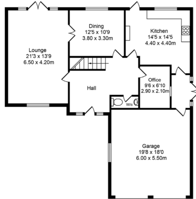
Ground Floor Approx. Floor Area 1286 Sq.Ft (119.5 Sq.M.)
