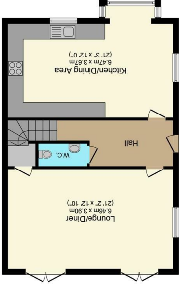
Floor area 63.2 m² (680 sq.ft.)
