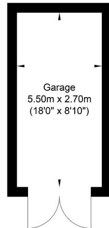
Garage Approximate Floor Area 159.84 sq ft (14.85 sq m)
