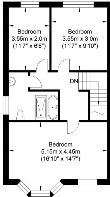
First Floor Approximate Floor Area 504.71 sq ft (46.89 sq m)
