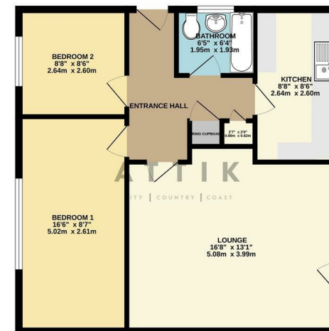
GROUND FLOOR 647 sq.ft. (60.1 sq.m.) approx.
