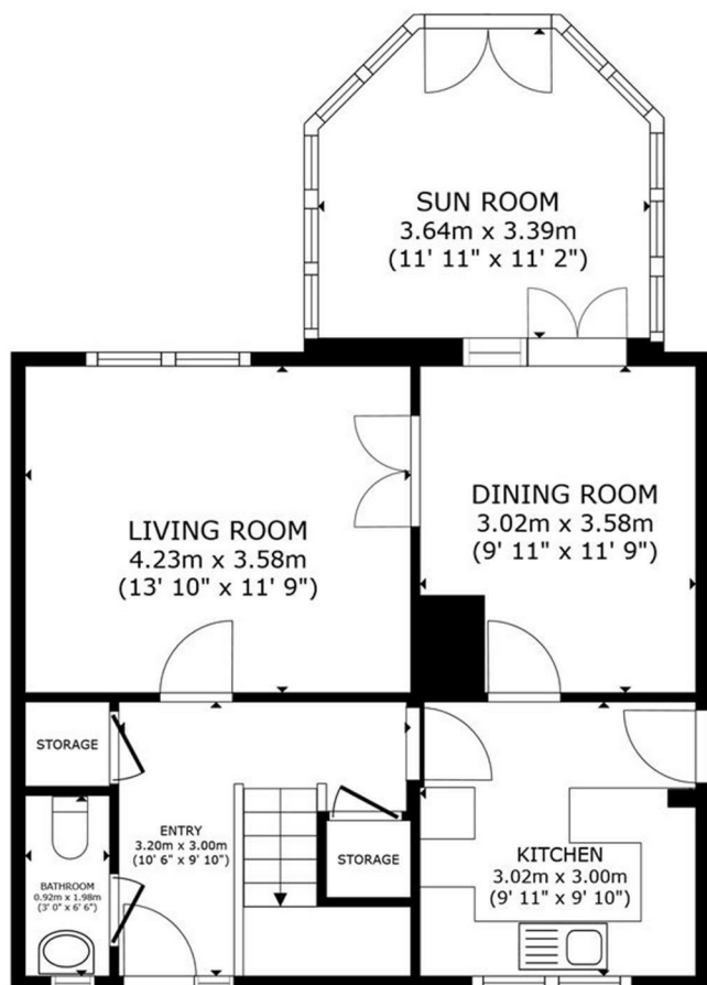
FLOOR 1
