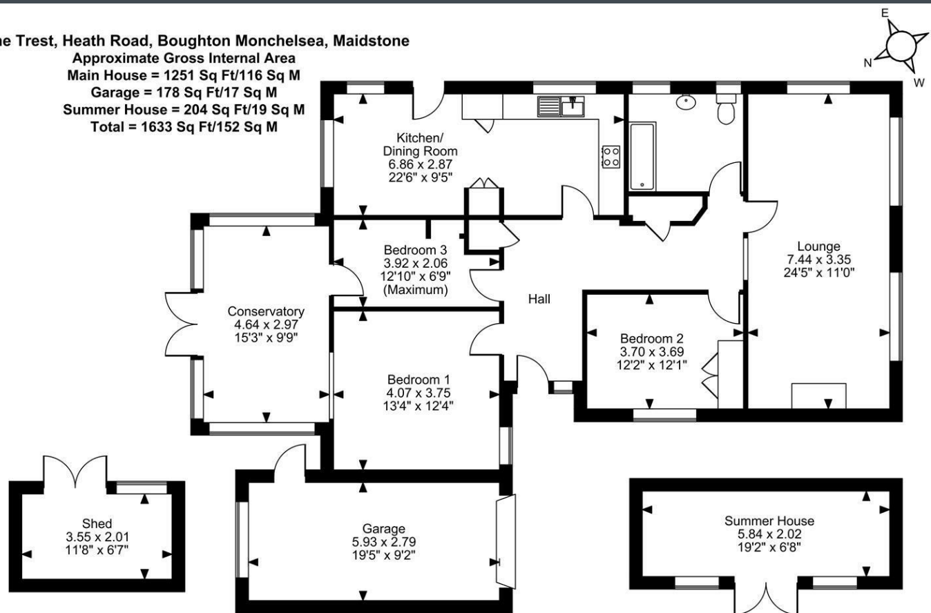
Ground Floor
