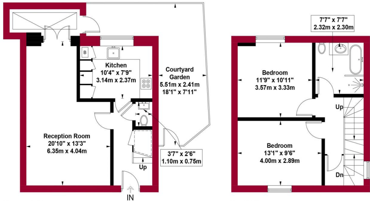
Ground Floor Gross Internal Floor Area 461 sq ft / 42.8 sq m
