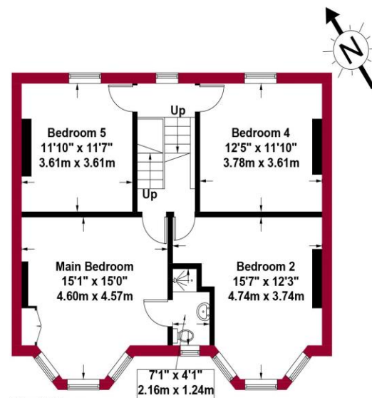
First Floor Gross Internal Floor Area 782 sq ft / 72.7 sq m
