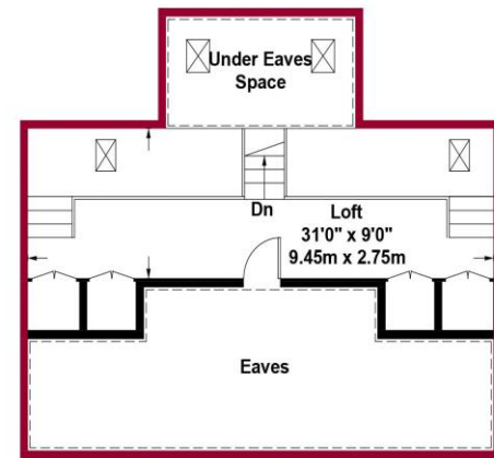
Loft Gross Internal Floor Area 684 sq ft / 63.6 sq m
