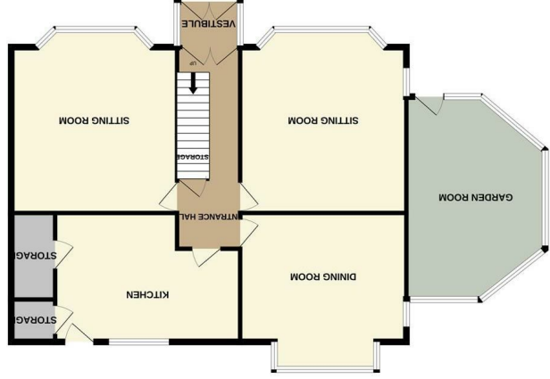
GROUND FLOOR (110.5 sq.m.) approx.
