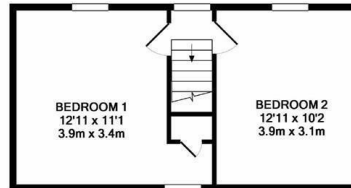
1ST FLOOR
