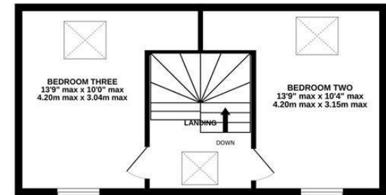
2ND FLOOR 414 sq.ft. (38.5 sq.m.) approx.
