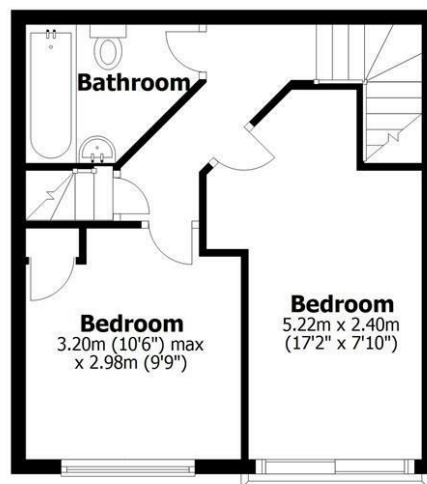
First Floor Approx. 33.1 sq. metres (355.9 sq. feet)
