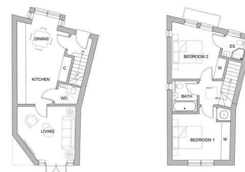
Ground Floor and First Floor Plans
