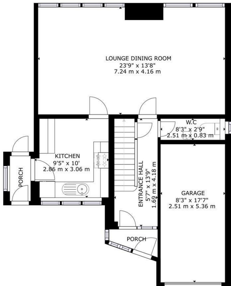
FLOOR 1
