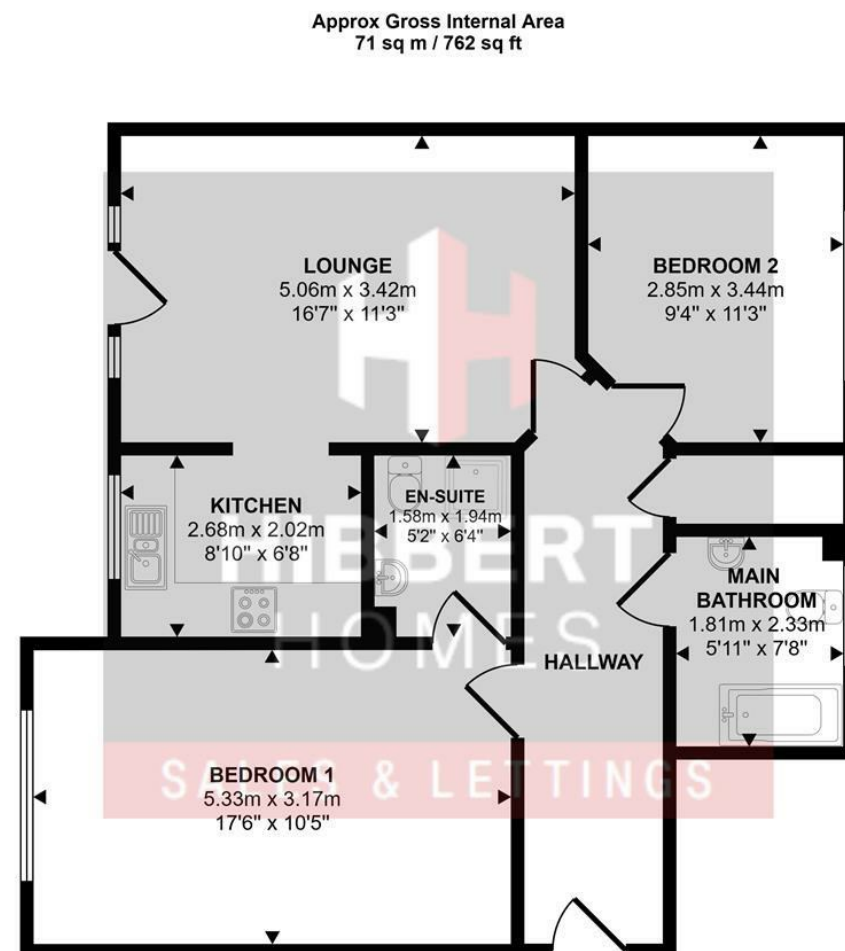
Floorplan
