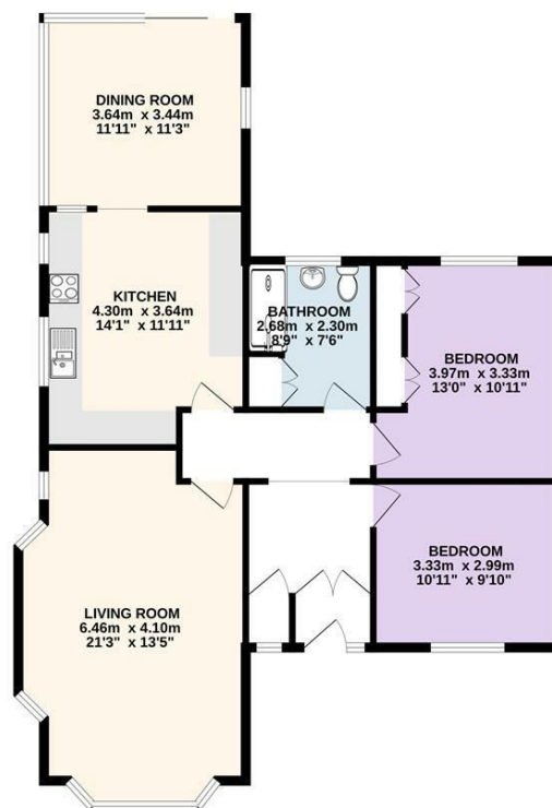
GROUND FLOOR 91.6 sq.m. (986 sq.ft.) approx.
