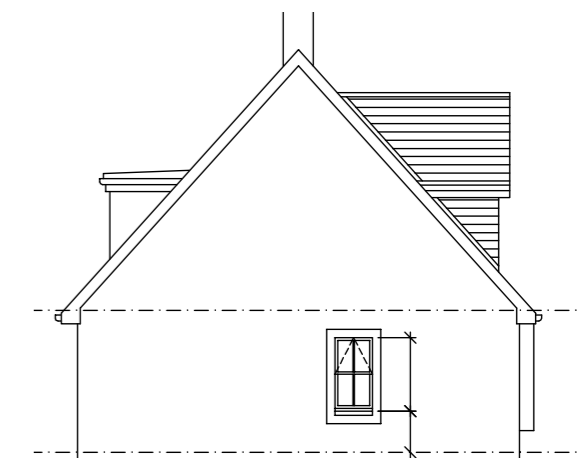
Gable Elevation 2
