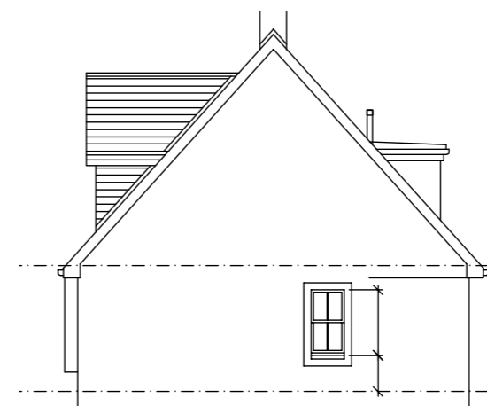
Gable Elevation 1
