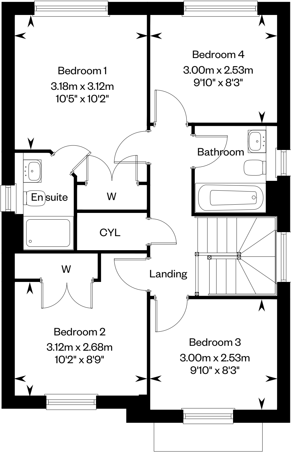
First floor
