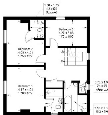
First Floor 65.2 sq m / 702 sq ft
