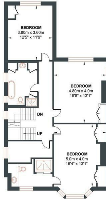
FIRST FLOOR Approximate Floor Area 942.59 sq ft (87.57 sq m)
