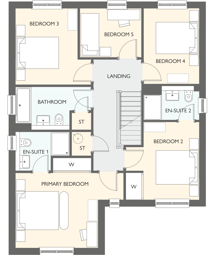
FIRST FLOOR
