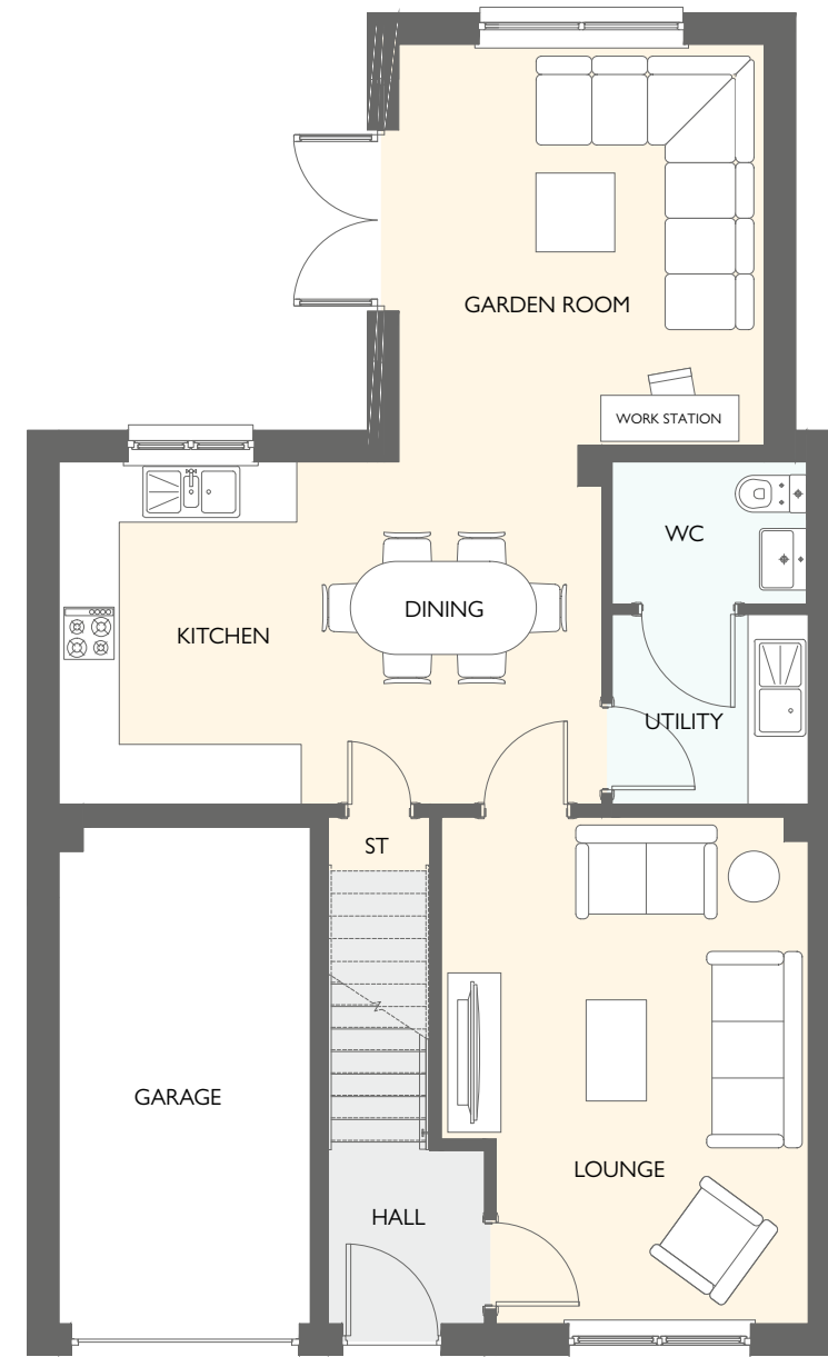
GROUND FLOOR
