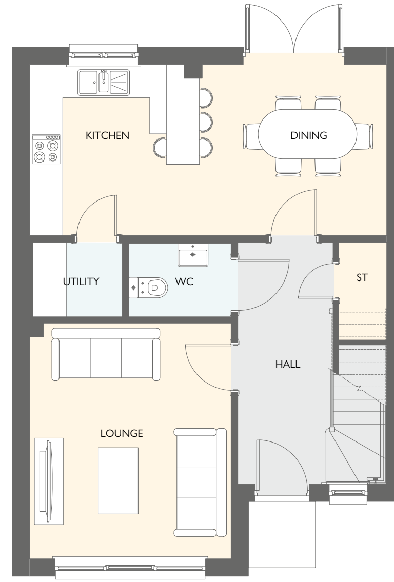
GROUND FLOOR
