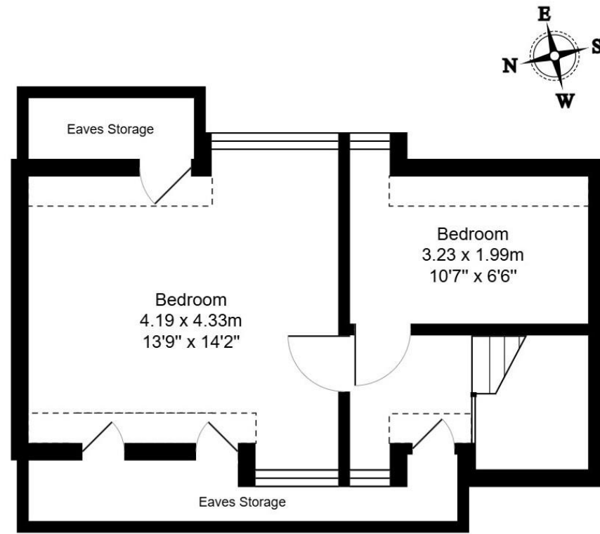
First Floor Area: 29.4 m 2 ... 316 ft 2
